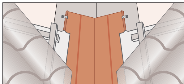
6. Limahoya
