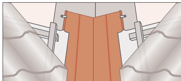
6. Limahoya
